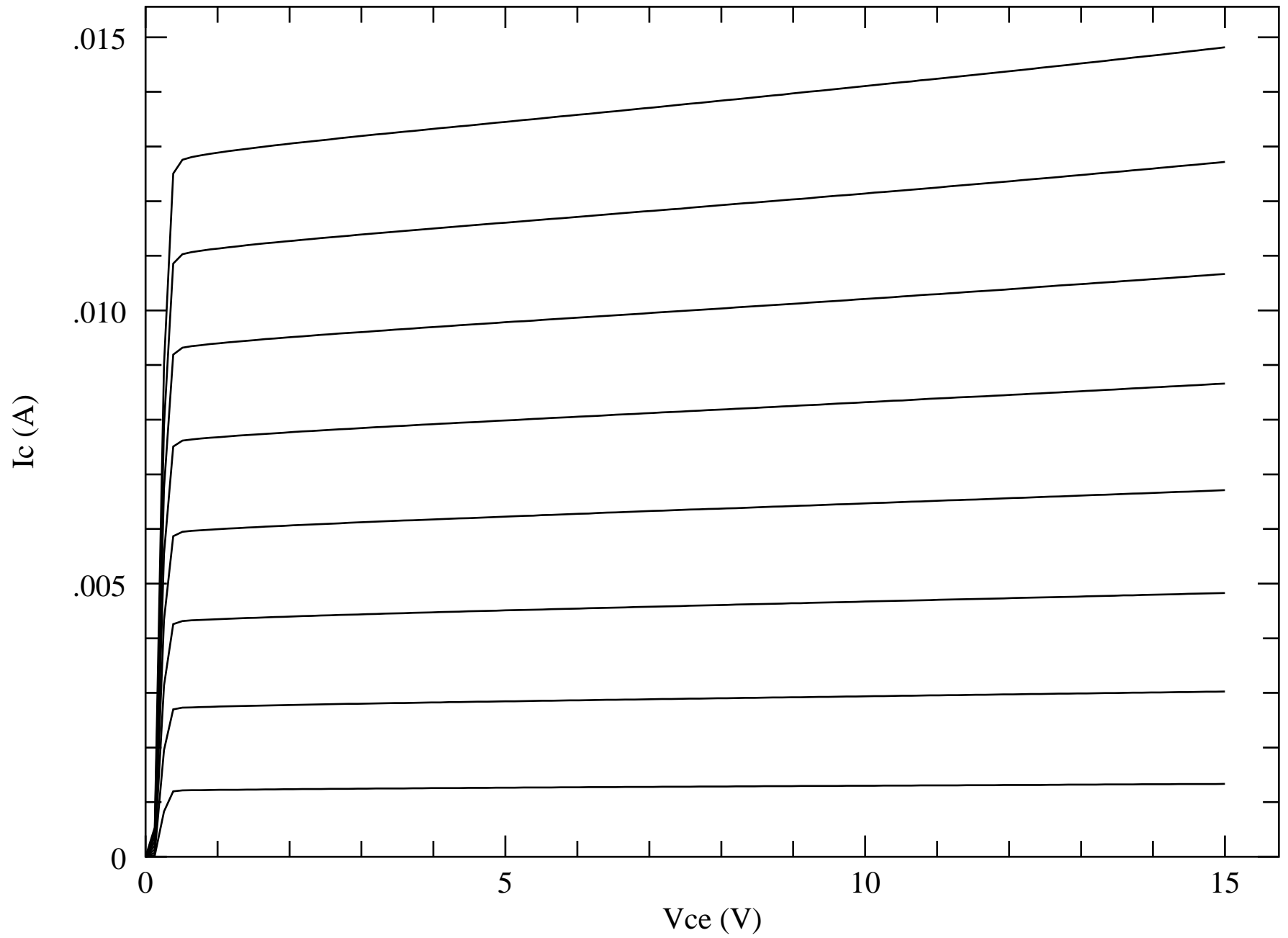
Characteristic Curves for NPN
