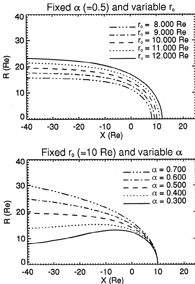
Figure 1. Graphical representation of equation (1). The radial distance r varies with r_0 and \alpha . The top panel shows fixed \alpha (=0.5) and variable r_0 . The bottom panel shows fixed r_0 (=10 R_e) and variable \alpha . Note that R = \sqrt{Y_{GSE}^2 + Z_{GSE}^2} = \sqrt{Y_{GSM}^2 + Z_{GSM}^2} , which is independent of GSE and GSM coordinates.
