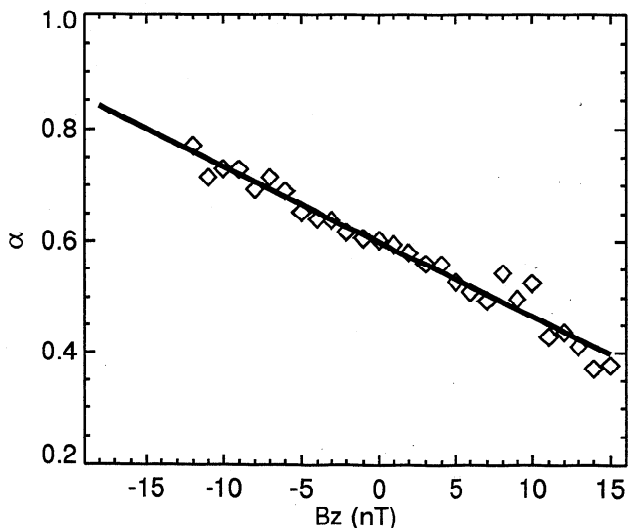
Figure 9. The same format as Figure 8, but using Roelof and Sibeck [1993] data.
