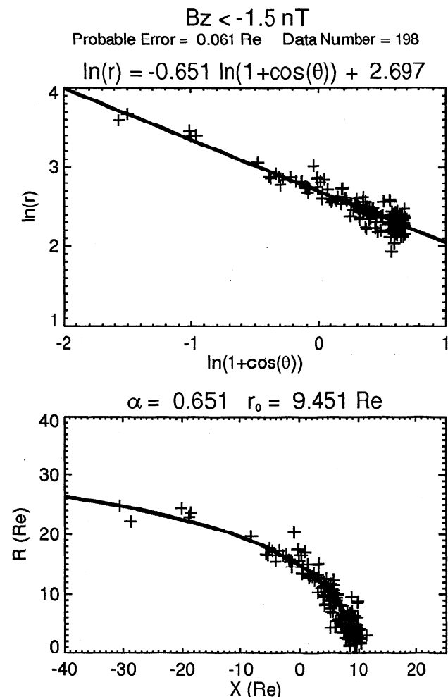
Figure 7. The same format as Figure 3, but for southward IMF data with normalization by D_p .
