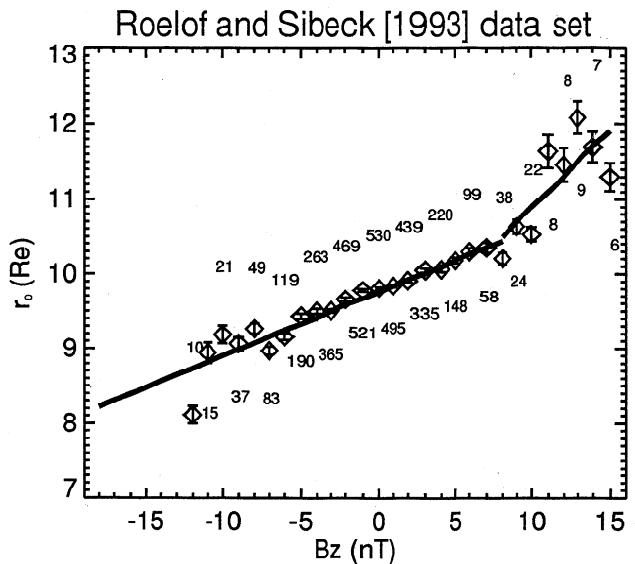
Figure 8. The variation of r_0 and \alpha with B_z . This relation is for D_p = 1.915 nPa. The diamond symbols represent the best-fit values of r_0 and \alpha . The error bar shows the probable error of the best-fit value. The solid lines show the fits. The number indicated above or below each error bar shows the number of data points for each bin.
