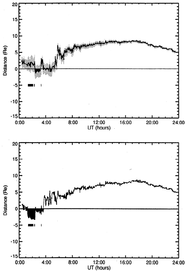
Figure 9. The distance from Interball to the predicted magnetopause in the same format as Figure 5. (top) Shue et al. [1997]. (bottom) Petrinec and Russell [1996].
