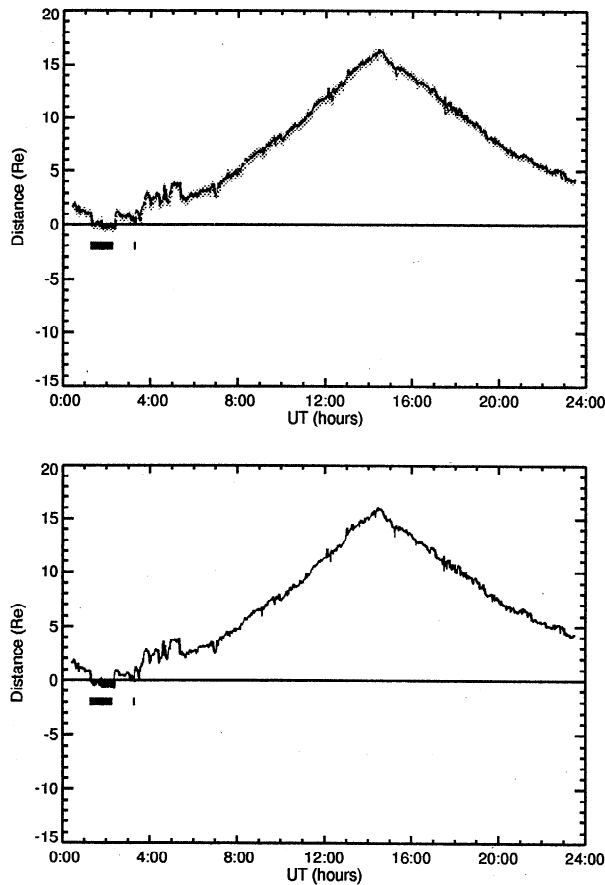
Figure 7. The distance from GMS 4 to the predicted magnetopause in the same format as Figure 5. (top) Shue et al. [1997]. (bottom) Petrinec and Russell [1996].
